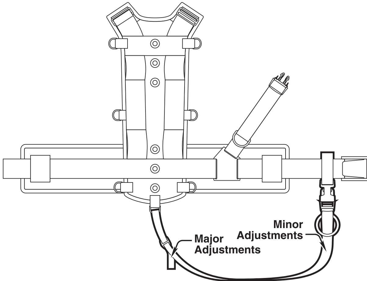
Figure 25: Crotch strap installation.
