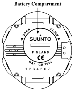
Fig. 6.1. Battery Compartment Lid
