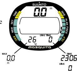
Fig. 3.5. Startup IV. Free mode. Depth and dive time are zero. Pressing +/- button activates alternative display of maximum depth and current time or dive number.
