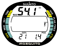
Fig. 3.21. Nitrox display. Maximum depth based on set O_2\% (21%) and PO_2 (1.4 bar) is 54.1 m [177 ft].
