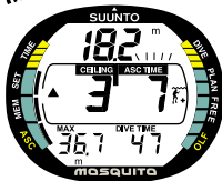
Fig. 3.17. Decompression dive, below floor. Upward pointing arrow, blinking ASC TIME label and an audible alarm tell you to ascend. Minimum total ascent time including safety stop is 7 minutes. Ceiling is at 3 m [10 ft].
