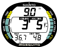
Fig. 3.18. Decompression dive, above floor. Upward pointing arrow has disappeared and ASC TIME label has stopped blinking, which means that you are in the decompression range.
