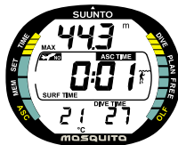
Fig. 3.26. Surface Mode after a violated decompression dive. ASC TIME symbol indicates that you have violated the ceiling for more than three minutes. The alternating display shows you that you must not dive again for at least 48 hours.
