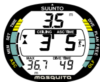
Fig. 3.19. Decompression dive, at ceiling zone. Two arrows point at each other (“hour glass”). You are in the optimum ceiling zone at 3.5 m [11 ft] and your minimum ascent time is 5 minutes.
