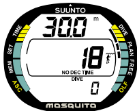
Fig. 3.9. Planning. The no-decompression time limit at 30.0 m [100 ft] is 18 minutes in P0/A0 mode..
