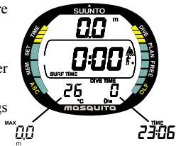
Fig. 3.4. Startup III. Surface mode (Air). Depth and dive time are zero. Pressing +/- button activates alternative display of maximum depth and current time.
