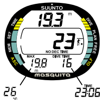
Fig. 3.11. Diving display. Present depth is 19.3 m [63 ft] and no-decompression stop time limit is 23 minutes in A0/P1 mode. Maximum depth during this dive has been 19.8 m [65 ft], elapsed dive time is 16 minutes. Alternative display shows temperature and current time.
