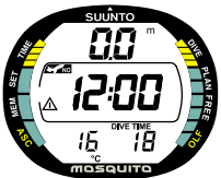
Fig. 3.25. Surface display. Alternating display showing the no-flying time.
