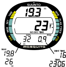
Fig. 3.22. Diving in EAN mode. The O_2\% is set to 32%. PO_2 is 0.9. Alternative displays are maximum depth, temperature, dive time and time.
